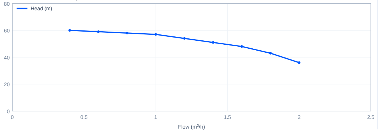
Head versus flow - CDL1-10, 50 Hz
