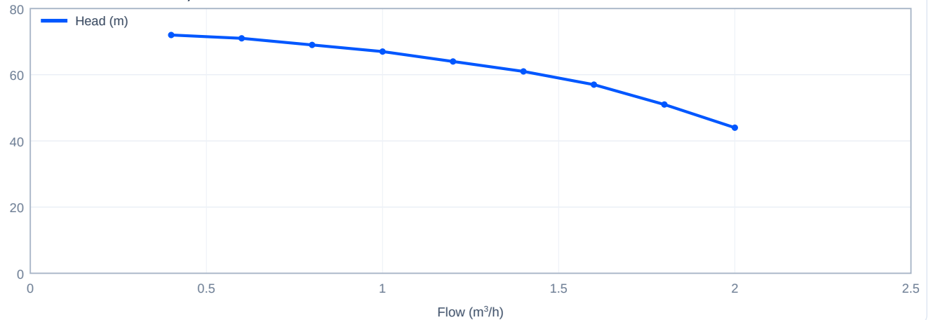
Head versus flow - CDL1-12, 50 Hz
