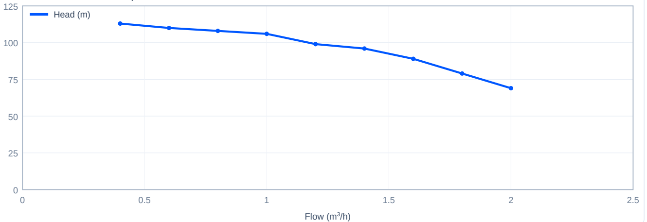
Head versus flow - CDL1-19, 50 Hz
