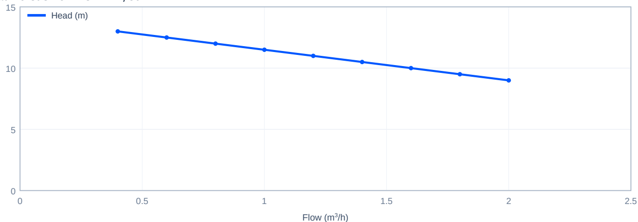
Head versus flow - CDL1-2, 50 Hz
