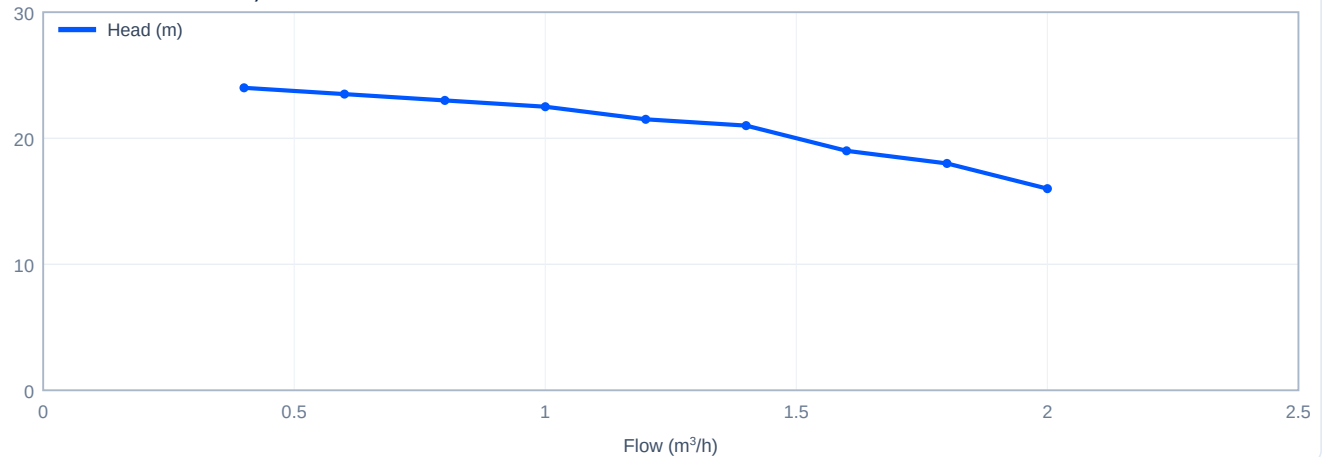
Head versus flow - CDL1-4, 50 Hz
