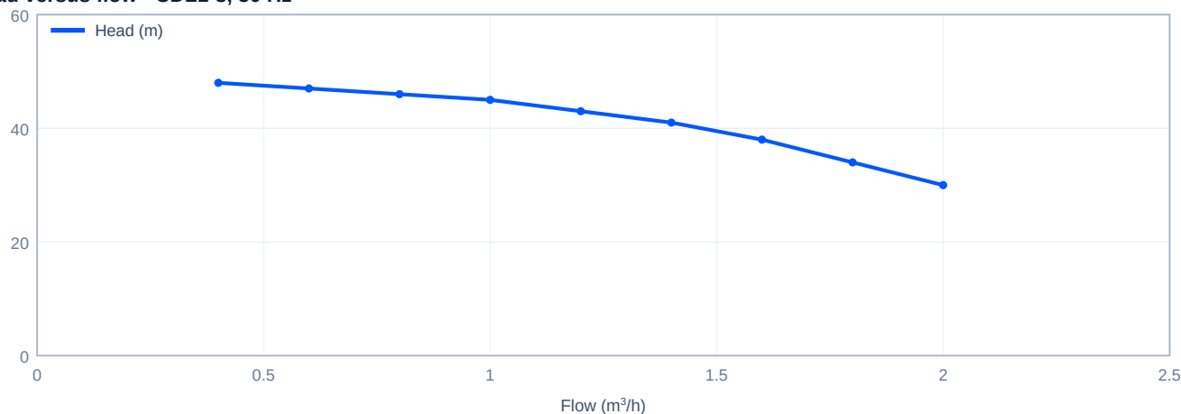
Head versus flow - CDL1-8, 50 Hz
