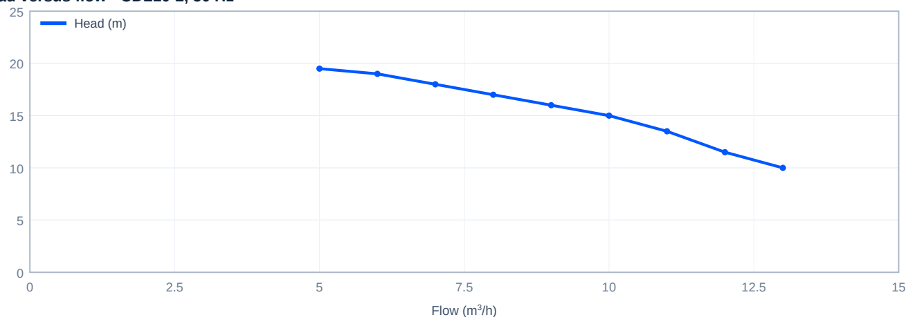
Head versus flow - CDL10-2, 50 Hz
