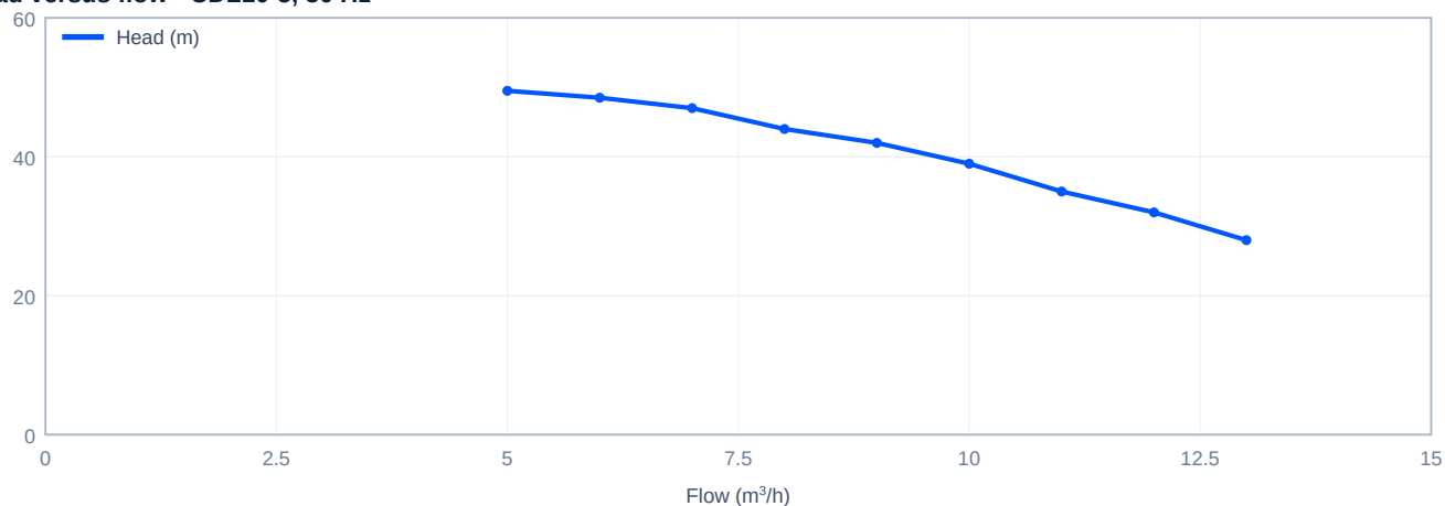
Head versus flow - CDL10-5, 50 Hz
