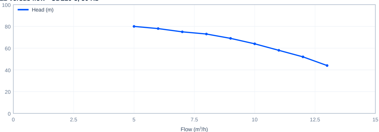
Head versus flow - CDL10-8, 50 Hz
