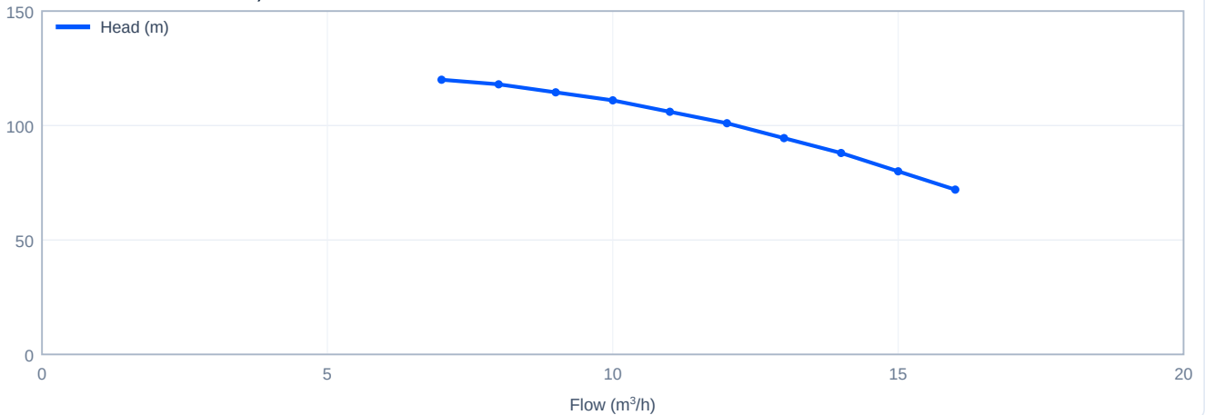
Head versus flow - CDL12-10, 50 Hz
