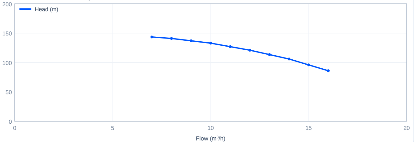
Head versus flow - CDL12-12, 50 Hz
