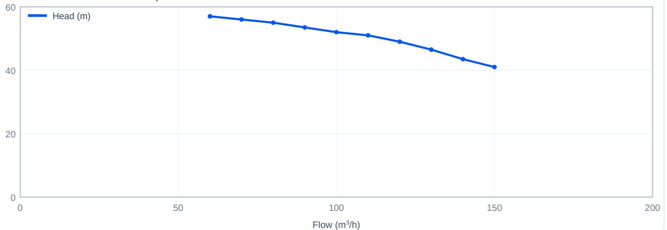
Head versus flow - CDL120-30-2, 50 Hz
