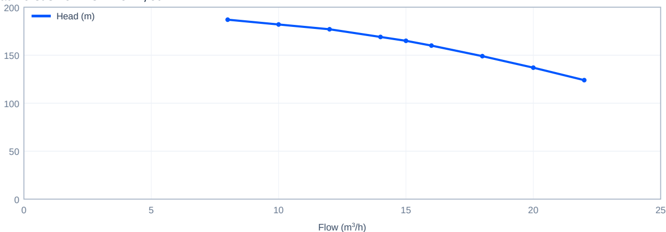
Head versus flow - CDL15-14, 50 Hz
