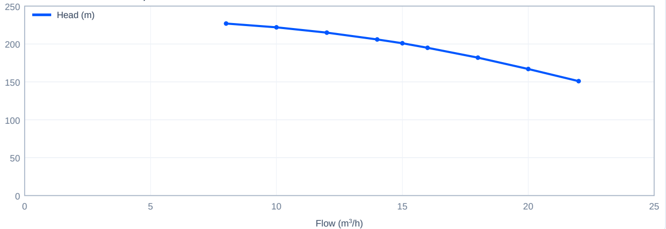
Head versus flow - CDL15-17, 50 Hz
