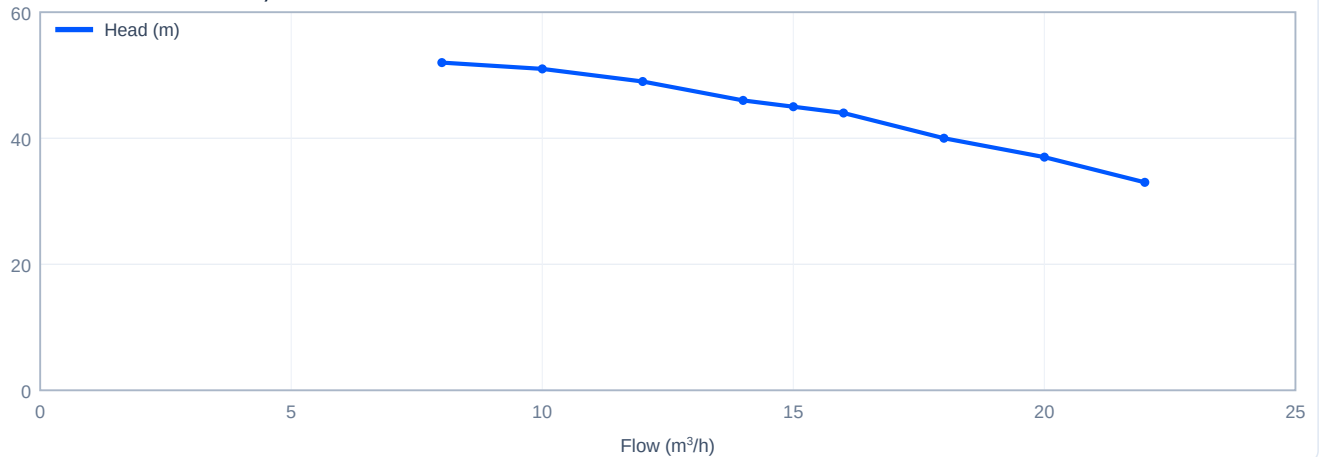
Head versus flow - CDL15-4, 50 Hz
