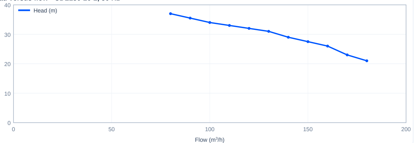
Head versus flow - CDL150-20-2, 50 Hz
