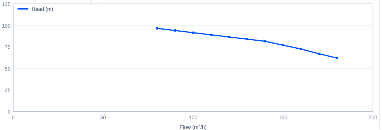
Head versus flow - CDL150-40-1, 50 Hz
