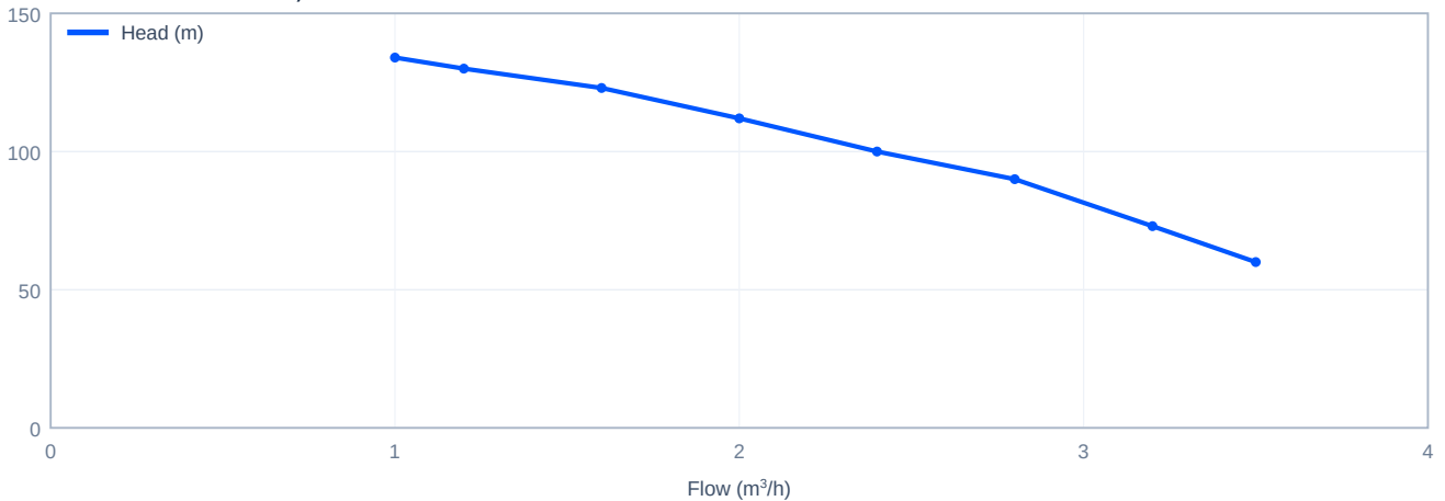
Head versus flow - CDL2-15, 50 Hz
