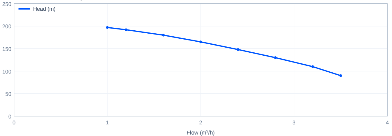
Head versus flow - CDL2-22, 50 Hz
