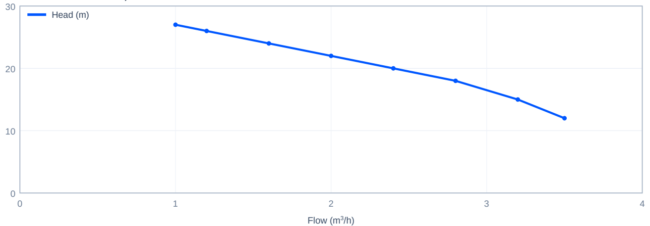
Head versus flow - CDL2-3, 50 Hz
