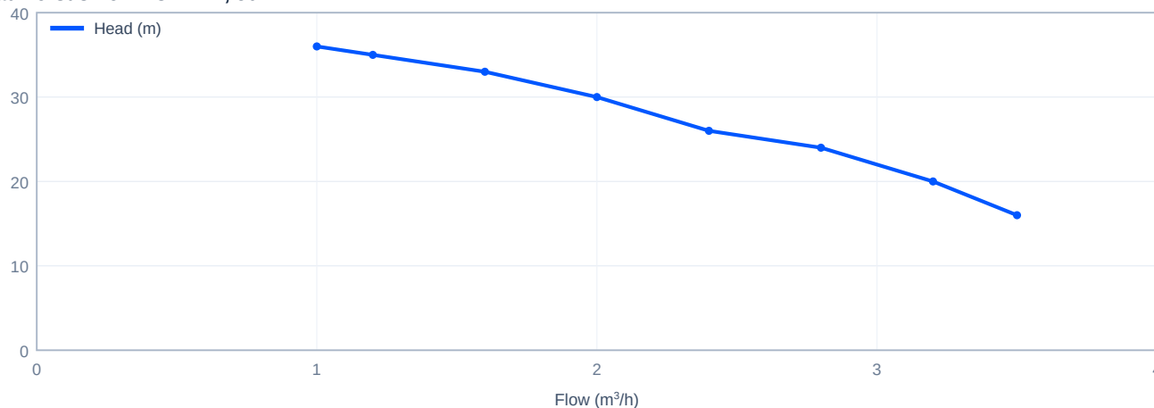
Head versus flow - CDL2-4, 50 Hz
