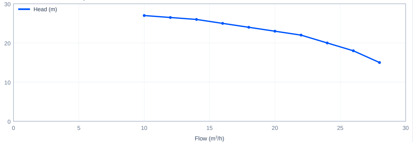
Head versus flow - CDL20-2, 50 Hz
