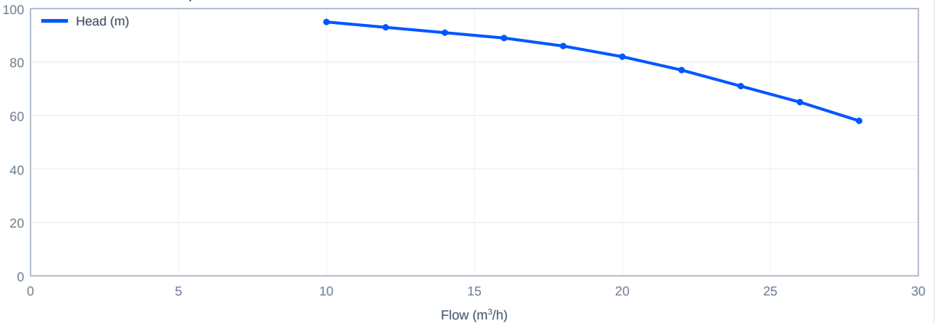
Head versus flow - CDL20-7, 50 Hz
