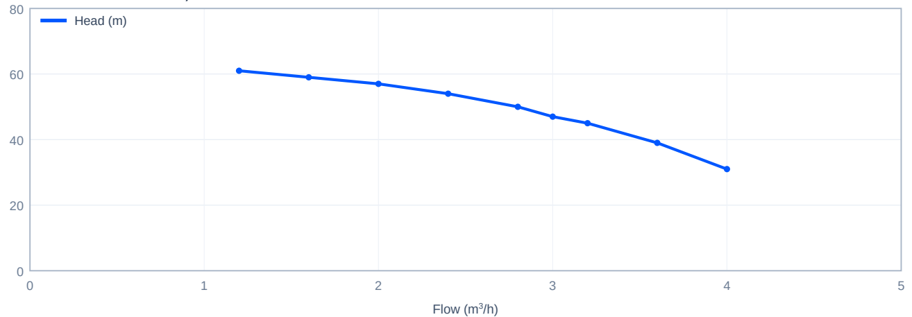
Head versus flow - CDL3-10, 50 Hz
