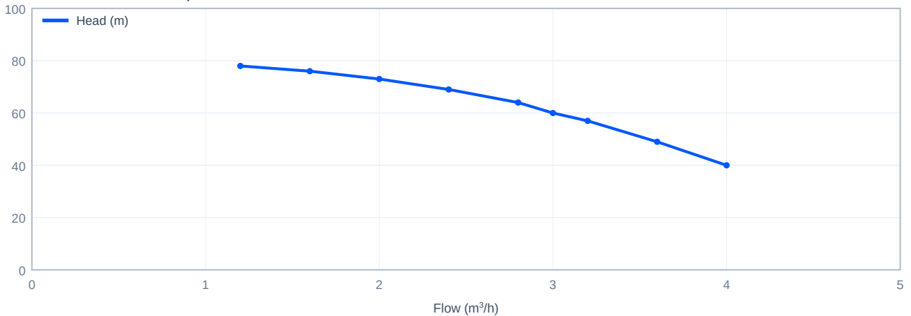
Head versus flow - CDL3-13, 50 Hz
