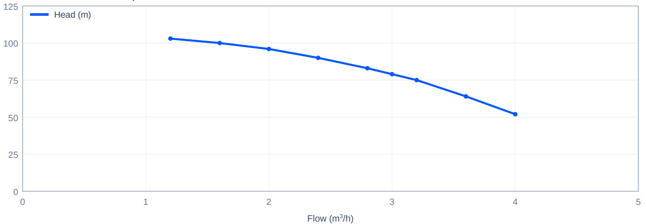
Head versus flow - CDL3-17, 50 Hz
