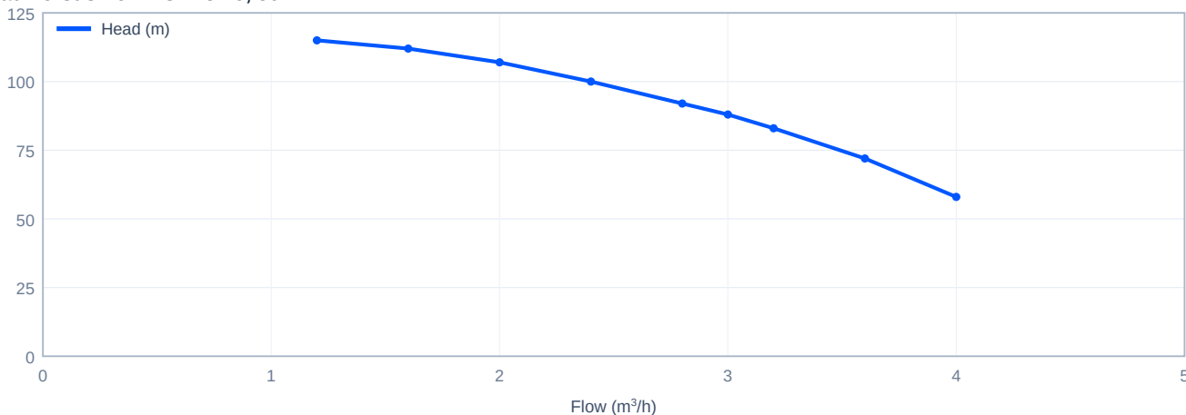
Head versus flow - CDL3-19, 50 Hz
