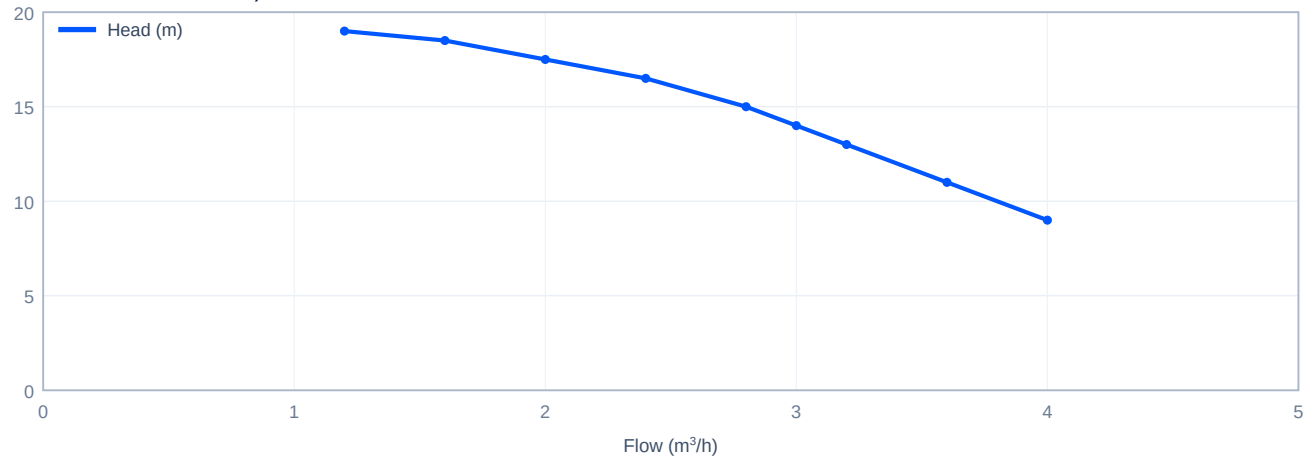
Head versus flow - CDL3-3, 50 Hz
