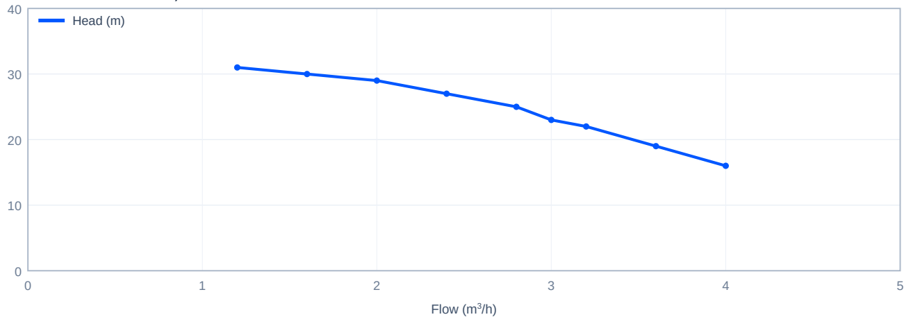
Head versus flow - CDL3-5, 50 Hz
