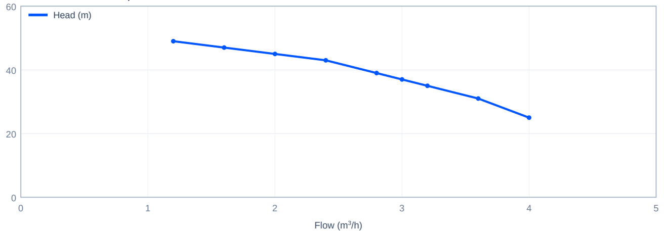
Head versus flow - CDL3-8, 50 Hz
