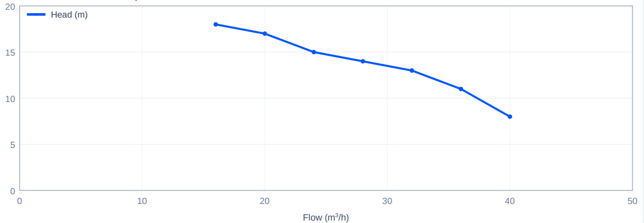
Head versus flow - CDL32-10, 50 Hz
