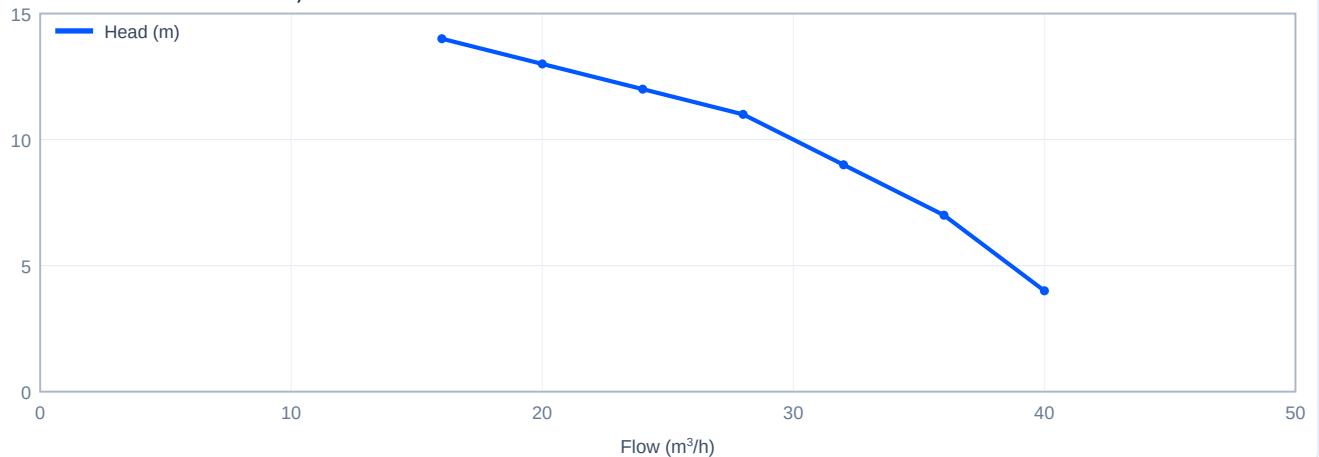
Head versus flow - CDL32-10-1, 50 Hz
