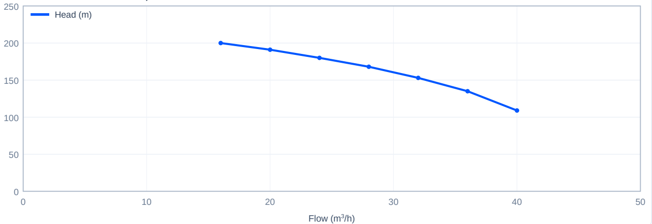
Head versus flow - CDL32-110, 50 Hz
