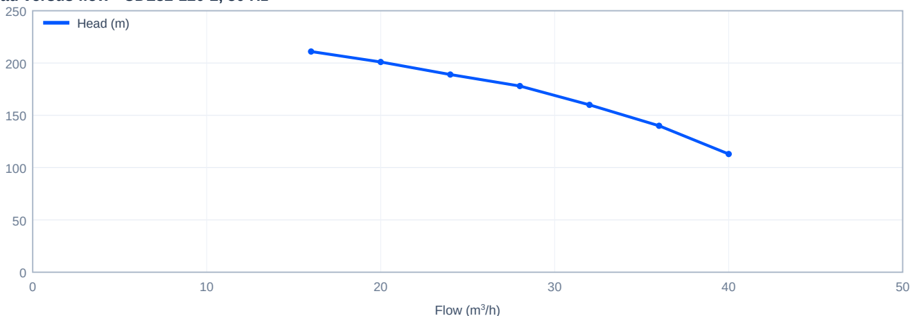
Head versus flow - CDL32-120-2, 50 Hz
