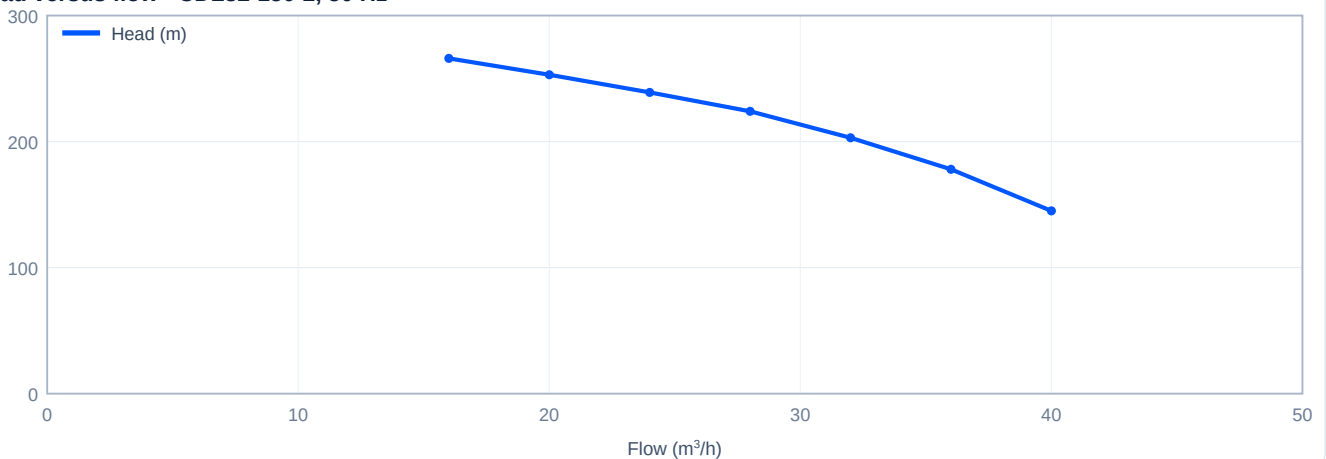
Head versus flow - CDL32-150-2, 50 Hz
