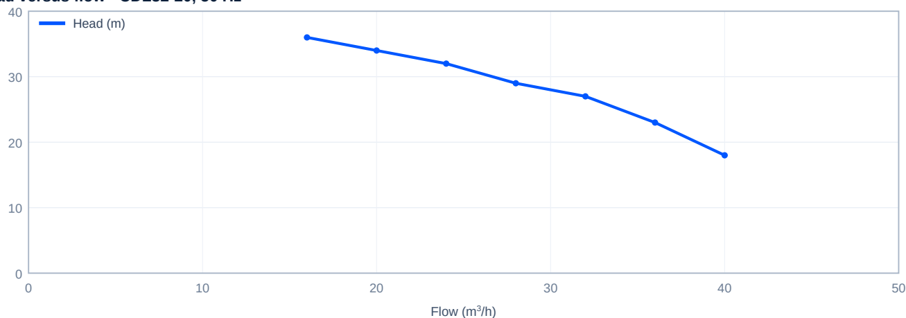
Head versus flow - CDL32-20, 50 Hz
