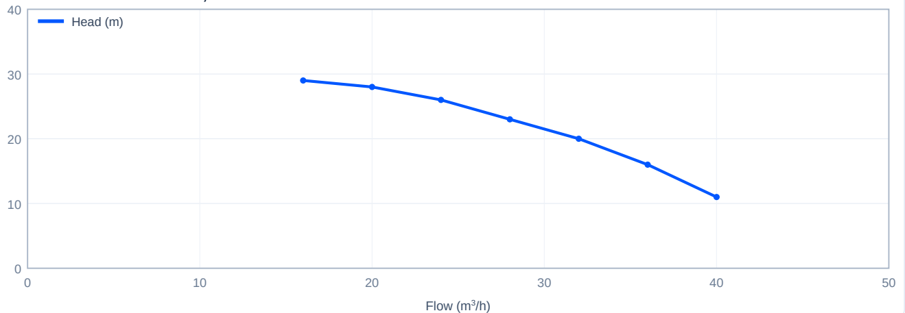
Head versus flow - CDL32-20-2, 50 Hz
