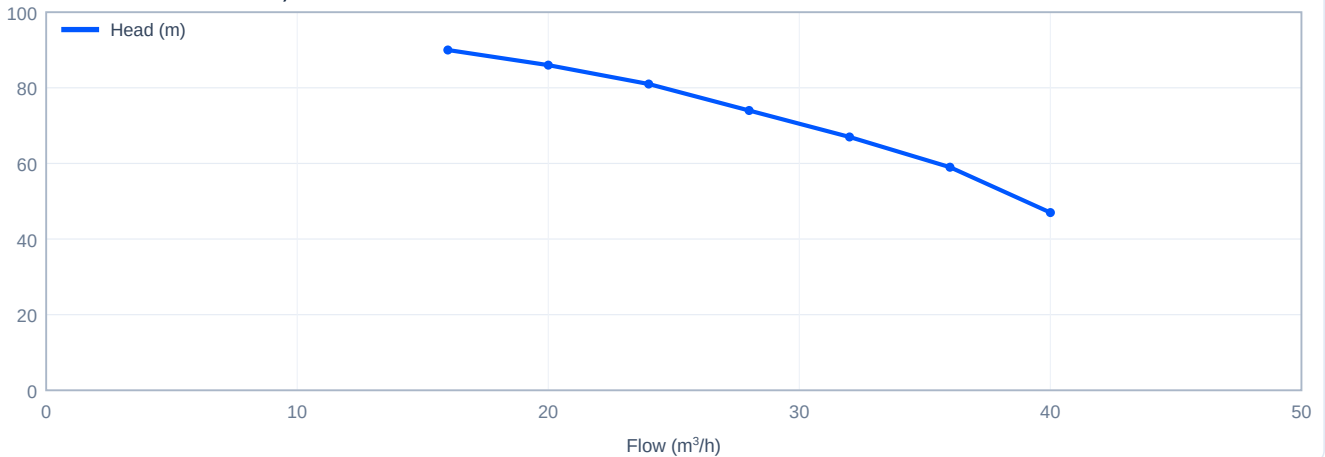
Head versus flow - CDL32-50, 50 Hz
