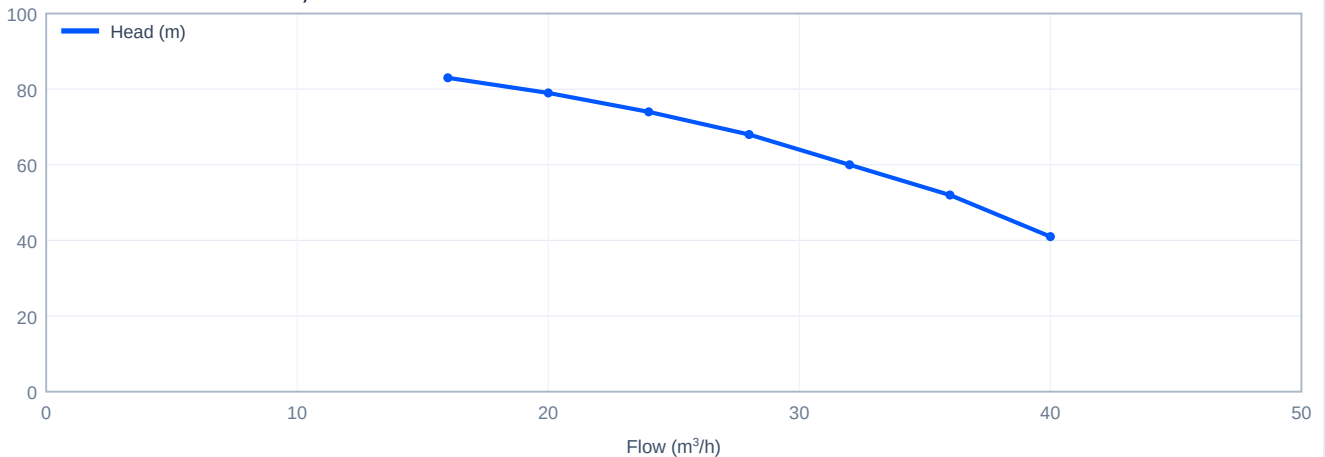
Head versus flow - CDL32-50-2, 50 Hz
