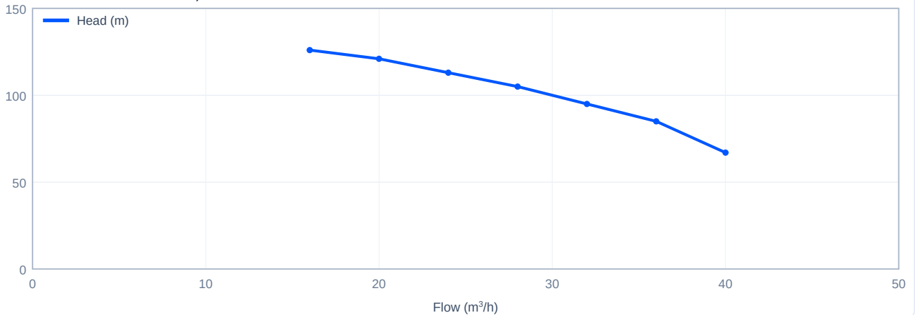
Head versus flow - CDL32-70, 50 Hz
