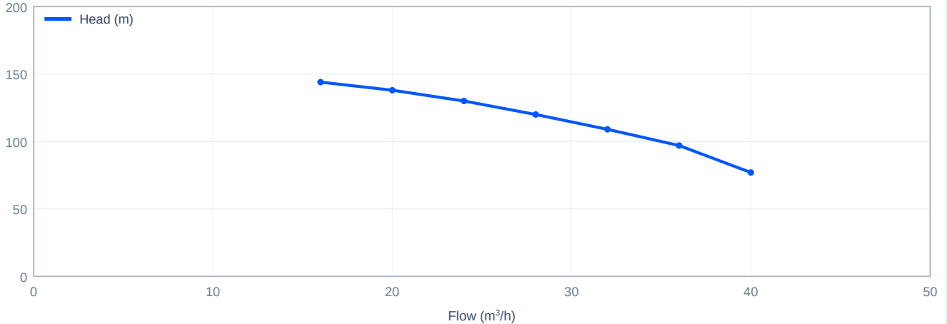
Head versus flow - CDL32-80, 50 Hz
