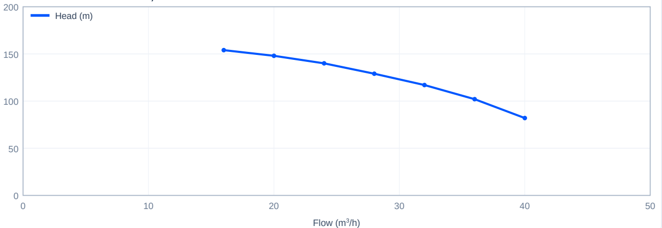
Head versus flow - CDL32-90-2, 50 Hz
