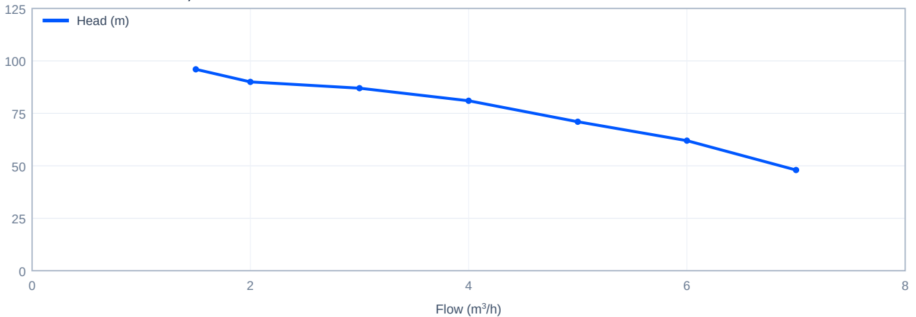
Head versus flow - CDL4-10, 50 Hz
