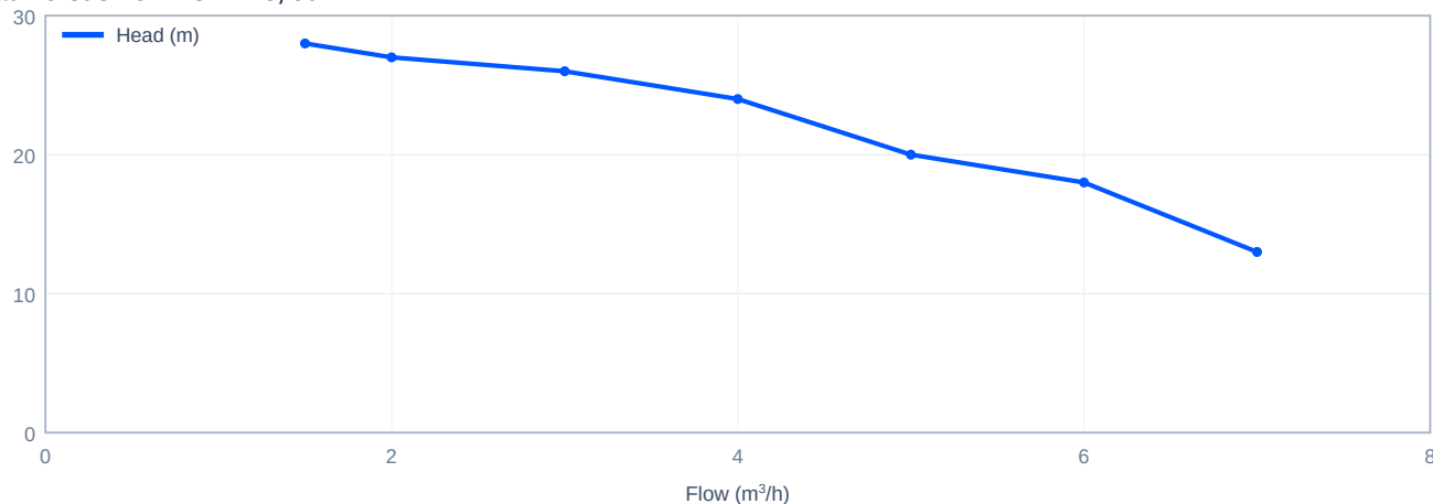
Head versus flow - CDL4-3, 50 Hz
