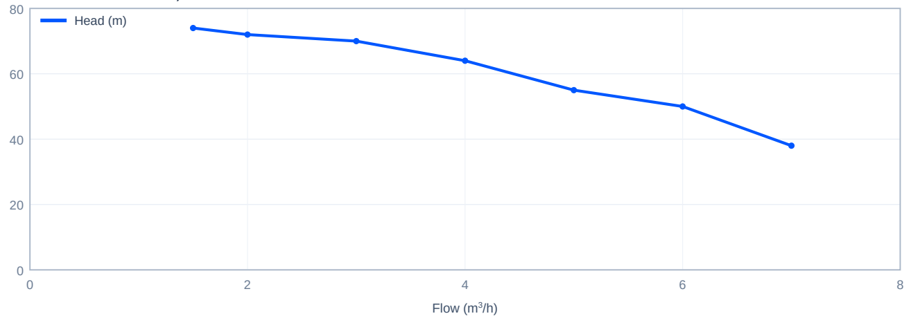
Head versus flow - CDL4-8, 50 Hz
