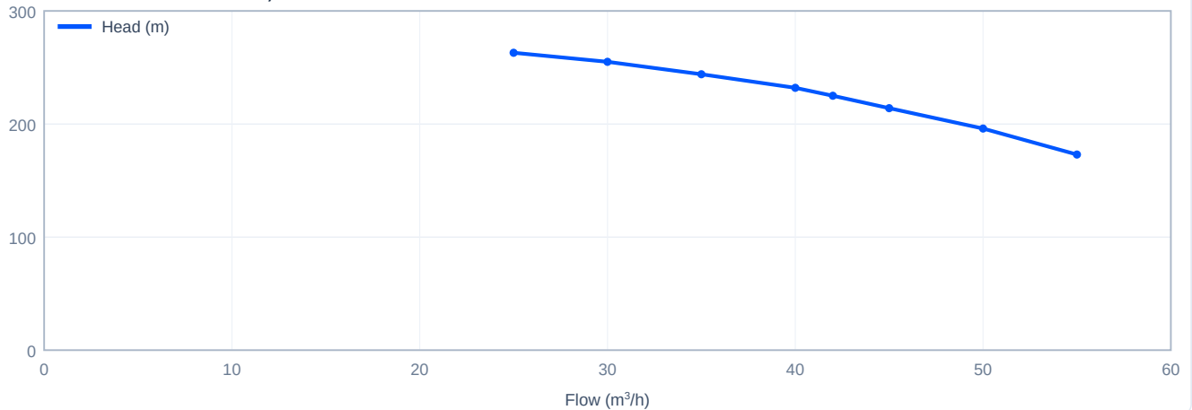
Head versus flow - CDL42-110, 50 Hz
