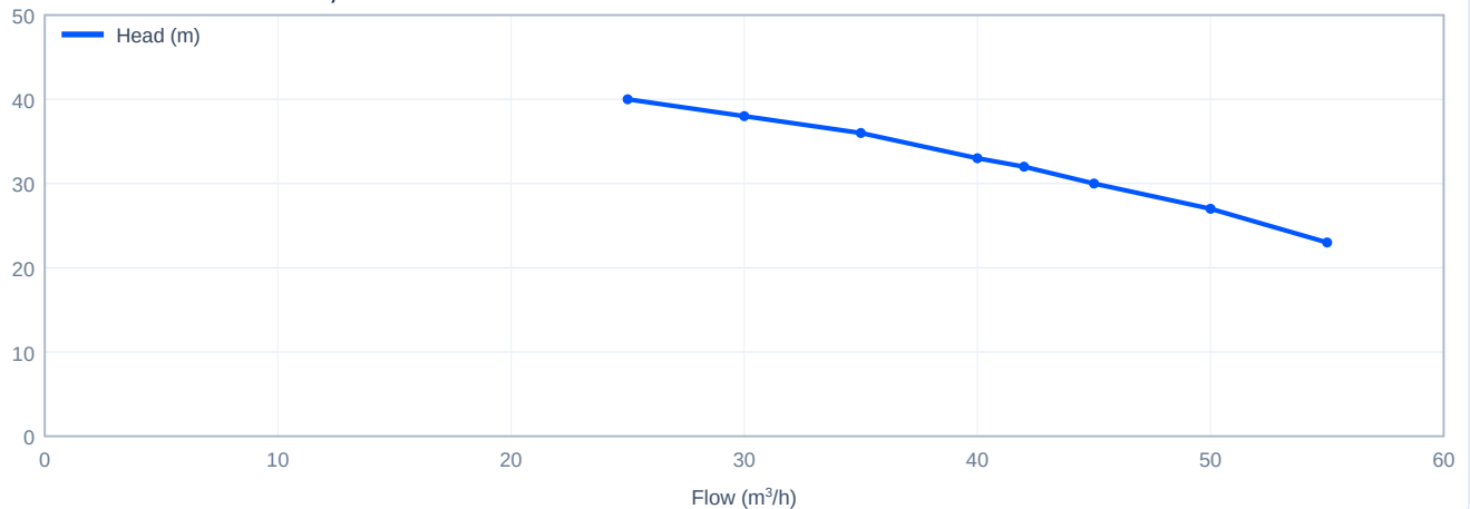
Head versus flow - CDL42-20-2, 50 Hz
