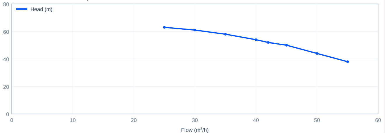
Head versus flow - CDL42-30-2, 50 Hz
