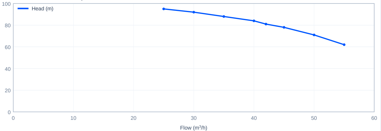
Head versus flow - CDL42-40, 50 Hz
