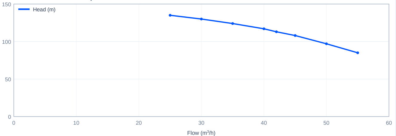
Head versus flow - CDL42-60-2, 50 Hz
